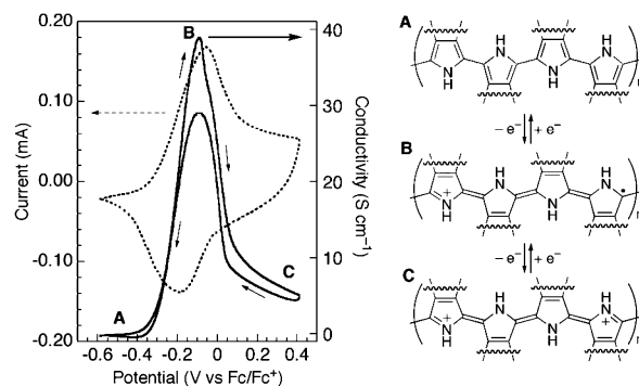
Figure 1. Cyclic voltammogram (25 mV/s; dotted line) and in situ conductivity measurement 7 (5 mV/s, offset potential of 40 mV; solid line) of poly( 2 ) on 5- \mu\text{m} interdigitated Pt electrodes in MeCN with 0.1 M (Bu 4 N)PF 6 as supporting electrolyte (left), and qualitative representations of neutral (A), polaronic (B), and bipolaronic (C) states of the polypyrrole backbone (right).
